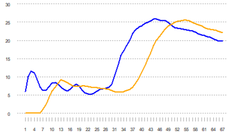
PRAM Disease (COVID Tests) 1-3 & 8-14 Rolling Daily Avg.
