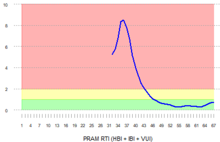
T2RPHD PRAM Resource Trend Index (RTI)
