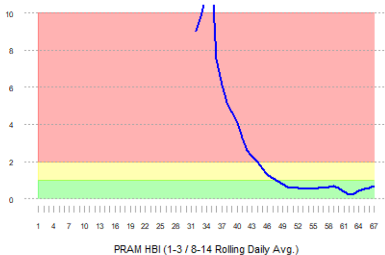
T2RPHD PRAM Hospital Beds Index (HBI)
