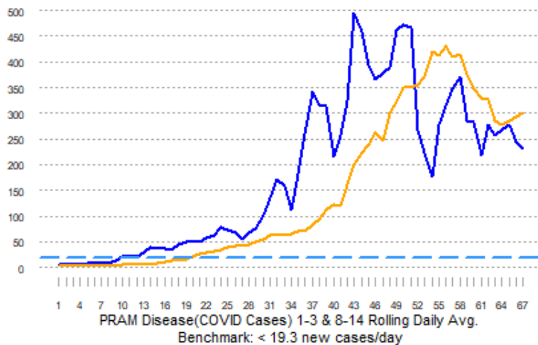
PRAM COVID Daily Rolling Average Nebraska New Cases
