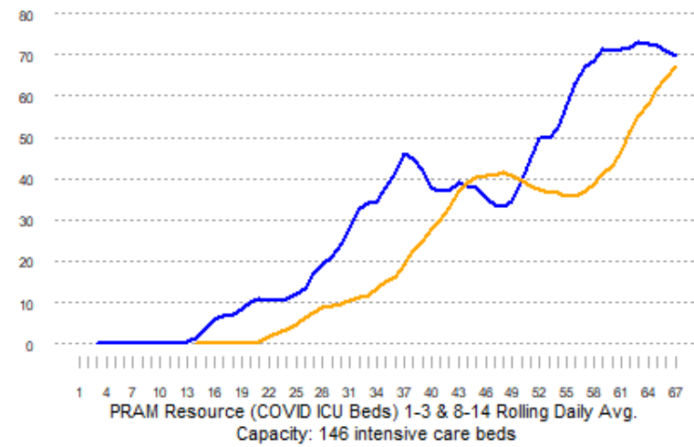
PRAM COVID Daily Rolling Average Nebraska Current ICU Beds
