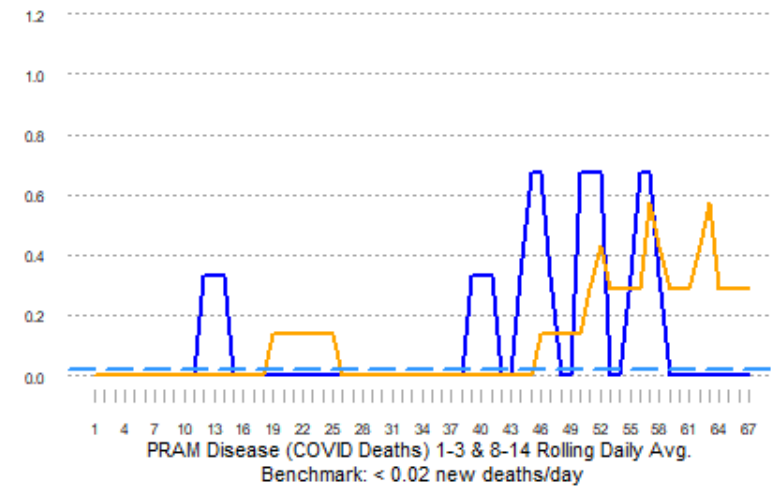
PRAM COVID Daily Rolling Average T2RPHD New Deaths
