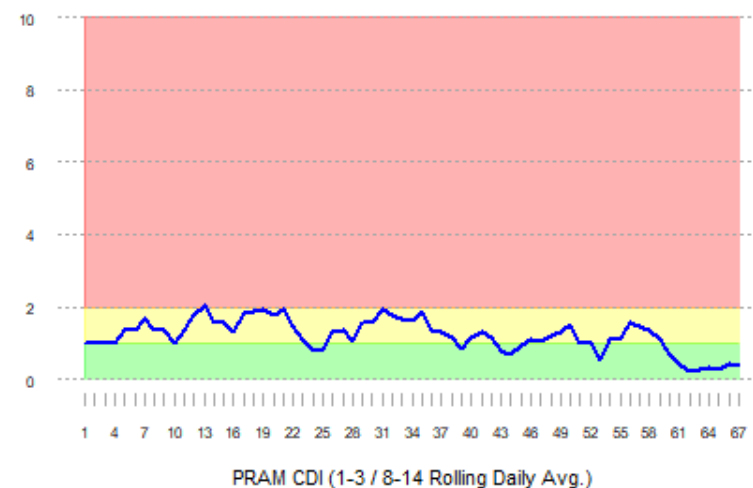
Nebraska PRAM Confirmed Death Index (CDI)
