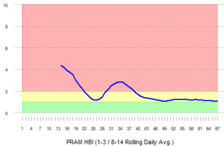
Nebraska PRAM Hospital Beds Index (HBI)
