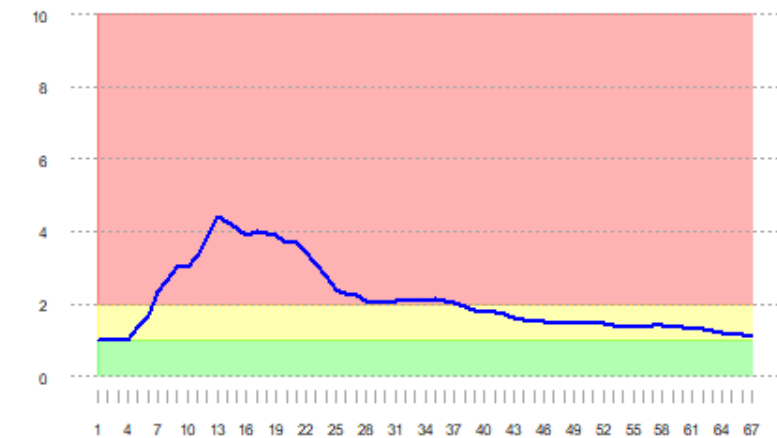
PRAM Disease (COVID Deaths) 1-3 / 8-14 Rolling Daily Avg.
