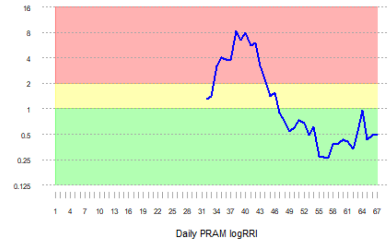
T2RPHD PRAM Log2 Recovery Ratio Index (logRRI)
