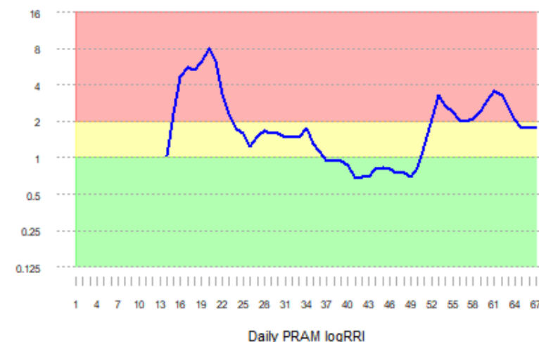
Nebraska PRAM Log2 Recovery Ratio Index (logRRI)
