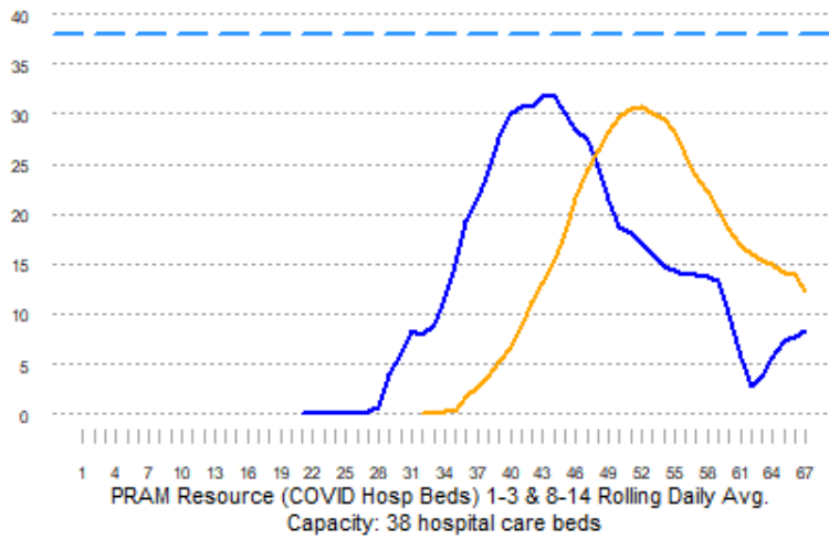
PRAM COVID Daily Rolling Average T2RPHD Current Hospital Beds
