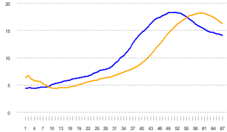
PRAM Disease (COVID Tests) 1-3 & 8-14 Rolling Daily Avg.
