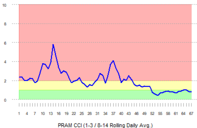
Nebraska PRAM Confirmed Case Index (CCI)
