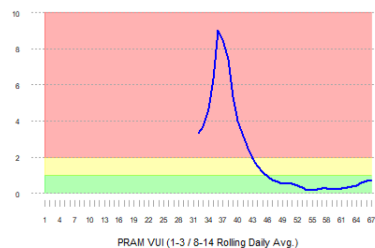
T2RPHD PRAM Ventilator Use Index (VUI)
