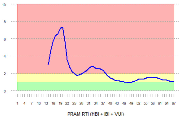
Nebraska PRAM Resource Trend Index (RTI)
