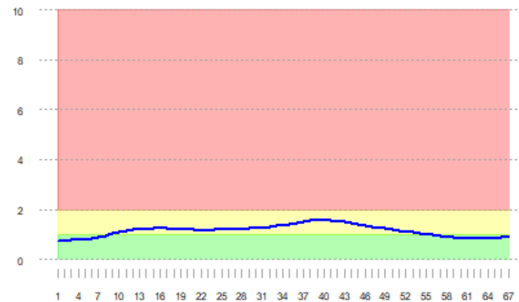
PRAM CPPTI (1-3 / 8-14 Rolling Daily Avg.)
