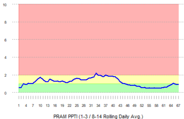
Nebraska PRAM Percent Positive Test Index (PPTI)
