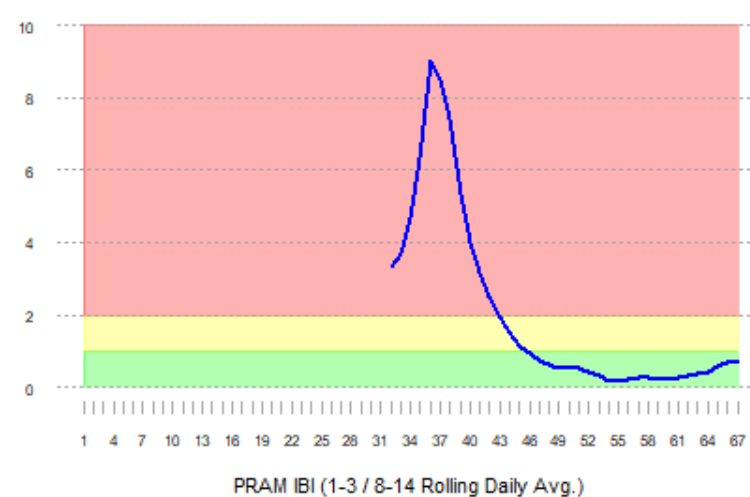
T2RPHD PRAM ICU Beds Index (IBI)
