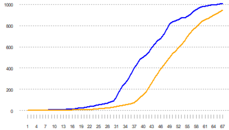
PRAM Disease (COVID Cases) 1-3 & 8-14 Rolling Daily Avg.
