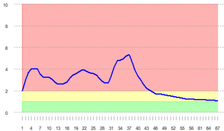
PRAM CHBI (1-3 / 8-14 Rolling Daily Avg.)
