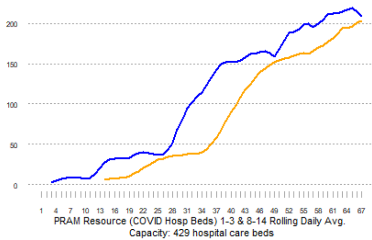
PRAM COVID Daily Rolling Average Nebraska Current Hospital Beds
