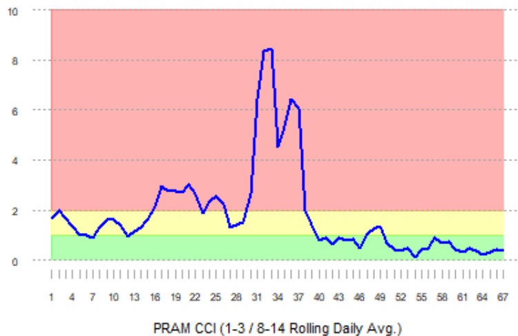
T2RPHD PRAM Confirmed Case Index (CCI)
