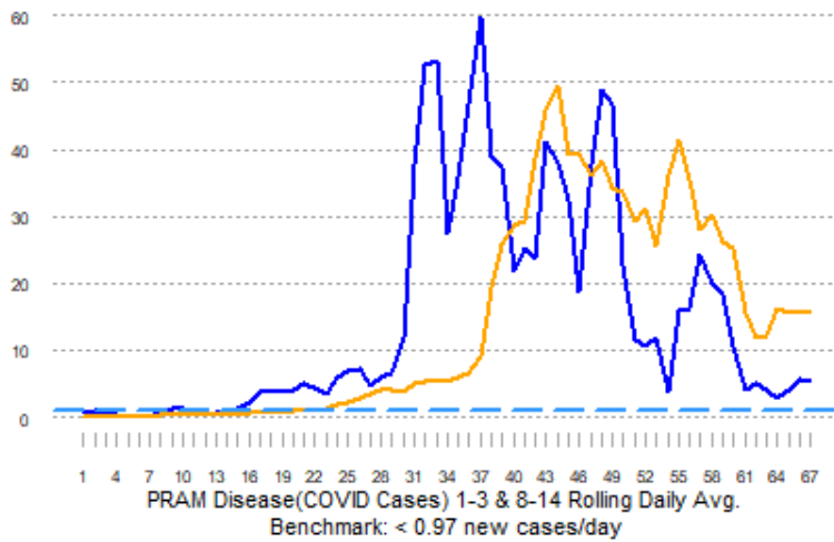
PRAM COVID Daily Rolling Average T2RPHD New Cases
