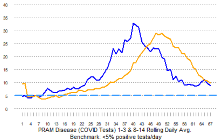
PRAM COVID Daily Rolling Average Nebraska Percent Positive Tests
