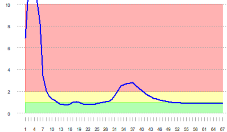
PRAM CPPTI (1-3 / 8-14 Rolling Daily Avg.)
