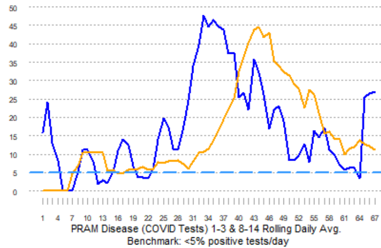
PRAM COVID Daily Rolling Average T2RPHD Percent Positive Tests
