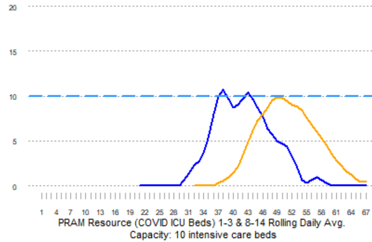
PRAM COVID Daily Rolling Average T2RPHD Current ICU Beds
