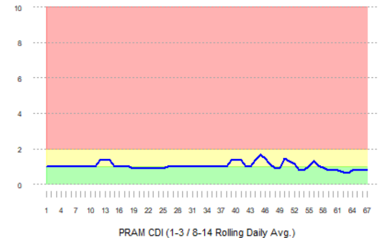
T2RPHD PRAM Confirmed Death Index (CDI)
