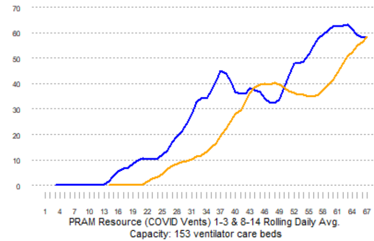
PRAM COVID Daily Rolling Average Nebraska Current Ventilators
