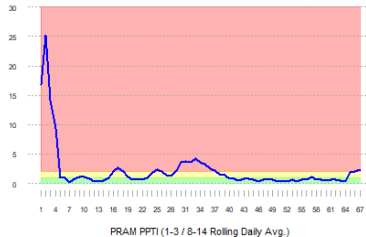
T2RPHD PRAM Percent Positive Test Index (PPTI)
