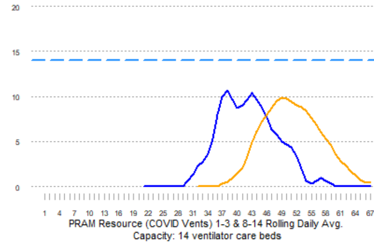
PRAM COVID Daily Rolling Average T2RPHD Current Ventilators
