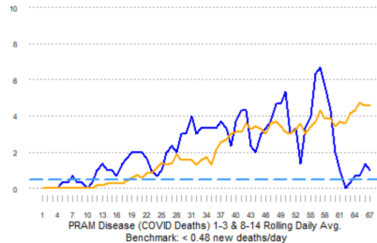
PRAM COVID Daily Rolling Average Nebraska New Deaths
